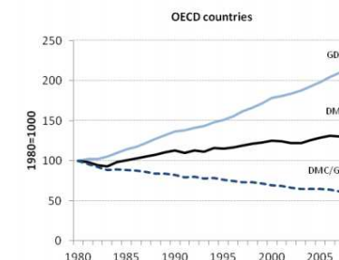
Figure 3. OECD material consumption versus GDP a
